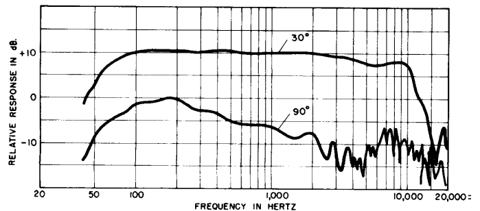
COMPARISON OF 30° AND 90° OFF-AXIS RESPONSE OF SM89 FIGURE 5
