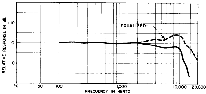
TYPICAL SM89 RESPONSE, 30° OFF-AXIS FIGURE 6
