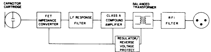
BLOCK DIAGRAM FIGURE 4
