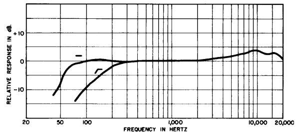
TYPICAL ON-AXIS FREQUENCY RESPONSE FIGURE 1
