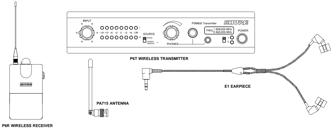
P6T Wireless Transmitter with rack-mounting hardware and one antenna P6R Wireless Body-Pack Receiver with antenna E1 Earpieces with foam ear inserts
