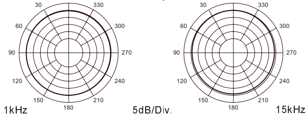
Polar Response
